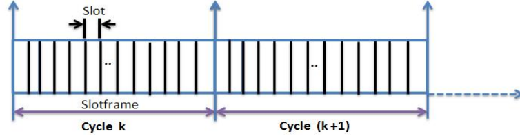
Figure 1: IEEE 802.15.4e TSCH slotframe
