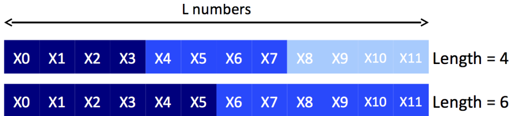
Figure 1: Sequence splitting in a unique original stream considering 2 processing elements (PEs), then 3 PEs
