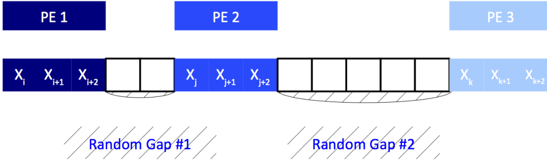
Figure 2: Random spacing applied to 3 processing elements (PEs)
