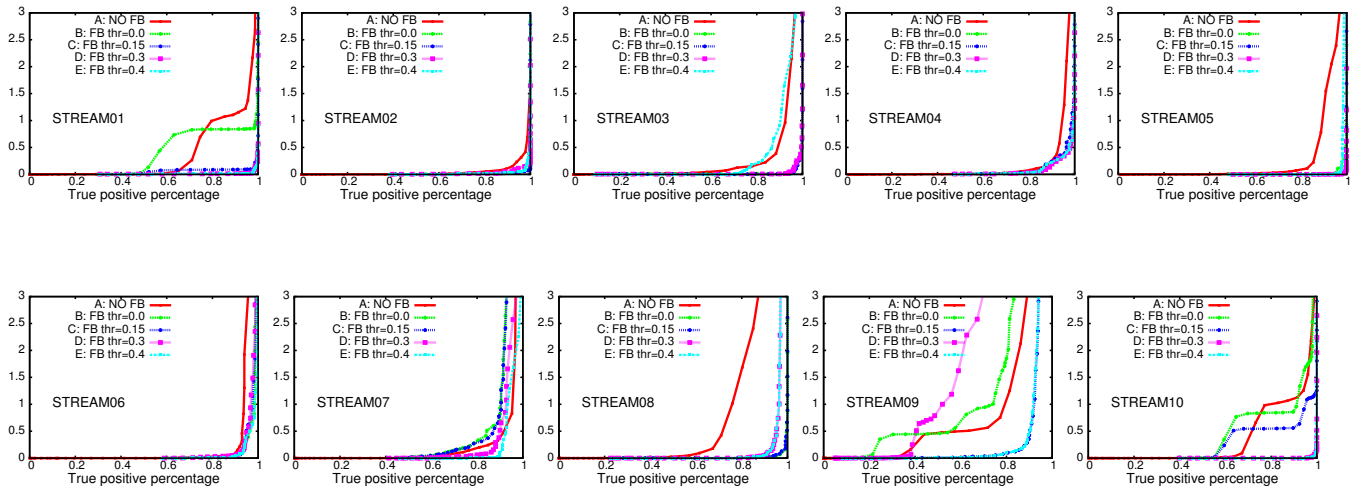
Fig. 4. Effect of dynamic attention priors on each of the 10 test streams. In each plot, there is either no feedback (A) or feedback where the tracker is fed only with detections that exceed confidence thresholds of 0 (B), 0.15 (C), 0.3 (D) and 0.4 (E). A strong overall improvement of detection rates is clearly observable.
