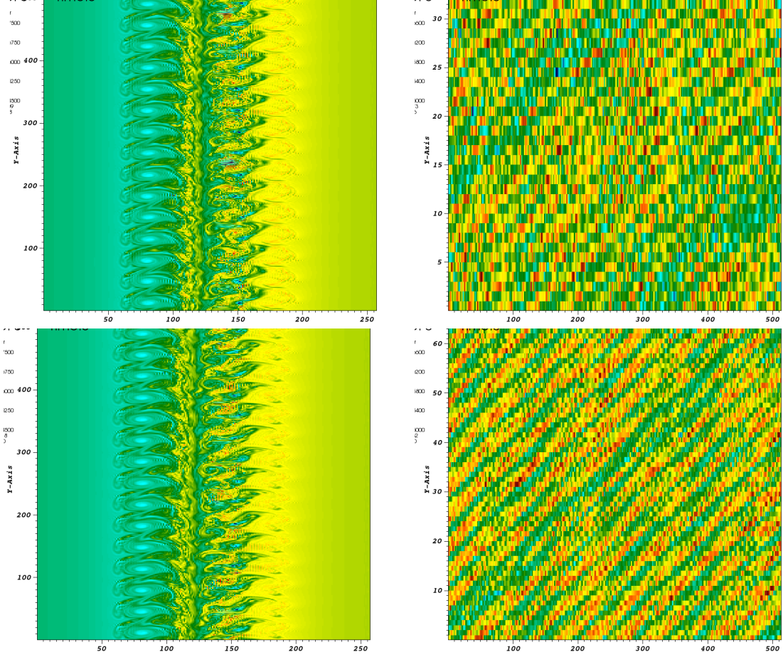
Figure 9: Poloidal cut (left) and \theta-z cut (right) of distribution function at time t = 6000 . Top: \iota = 0.8 , n = -11 , m = 15 on 256 \times 512 \times 32 \times 128 grid. Bottom: \iota = 0.8 , n = -11 , m = 15 on 256 \times 512 \times 64 \times 128 grid.
