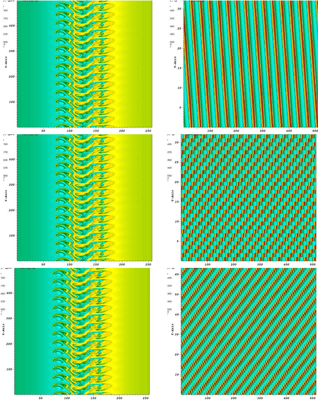
Figure 8: Poloidal cut (left) and \theta-z cut (right) of distribution function at time t = 4000 . Top: \iota = 0 , n = 1 , m = 15 on 256 \times 512 \times 32 \times 128 grid. Middle: \iota = 0.8 , n = -11 , m = 15 on 256 \times 512 \times 32 \times 128 grid. Bottom: \iota = 0.8 , n = -11 , m = 15 on 256 \times 512 \times 64 \times 128 grid.
