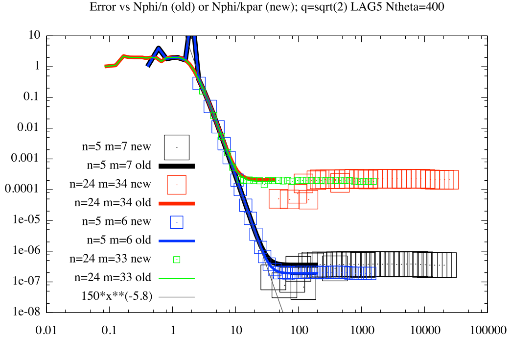
Figure 5: L^{\infty} error vs N_{\varphi}/n for the standard method (old) and vs N_{\varphi}/|k_{\parallel}| for the aligned method (new). Parameters are q = \sqrt{2} , N_{\theta} = 400 . Top: LAG3; bottom: LAG5.
