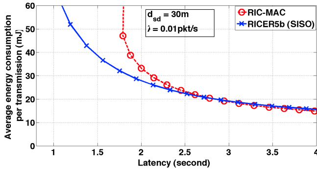
Fig. 4. Comparison of energy consumption between single-hop and cooperative relay using real MAC protocols (artificial energy model)
