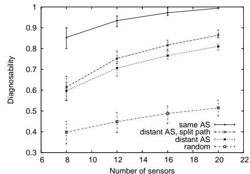
Figure 5: Sensor placement and diagnosability
