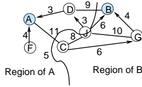
Figure 4: Example of the division of vertices into regions after deleting the edge CF .
