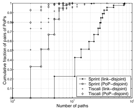
Figure 2: PoP-level path diversity in the Sprint and Tiscali topologies inferred by Rocketfuel.
