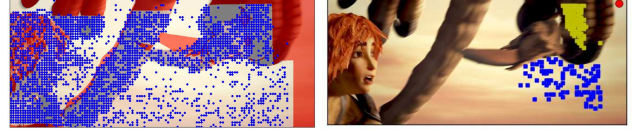
Figure 6. Left. Matches position returned by [35] are shown in blue. Red denotes occluded areas. Right. Yellow (resp. blue) squares correspond to the 100 nearest matches with a Euclidean (resp. edge-aware geodesic) distance for the pixel shown in red. All neighbor matches with a Euclidean distance holds to a different object while the geodesic distance allows to capture matches from the same region, even in the case of large occluded areas.
