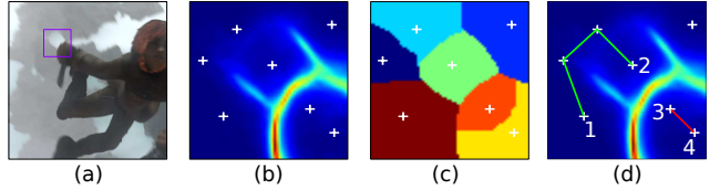
Figure 5. For the region shown in (a), (b) shows the image edges C and white crosses representing the match positions \{p_m\} . (c) displays the assignment L , i.e. geodesic Voronoi cells. We build a graph \mathcal{G} from L (see text). (d) shows the shortest path between two neighbor matches, which can go through the edge that connects them (3-4) or a shorter path found by Dijkstra’s algorithm (1-2).
