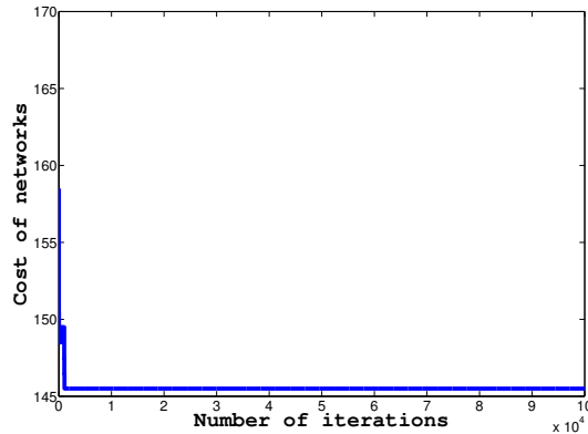
Figure 3: Sample path of network dynamics for \varepsilon = 0.00001
