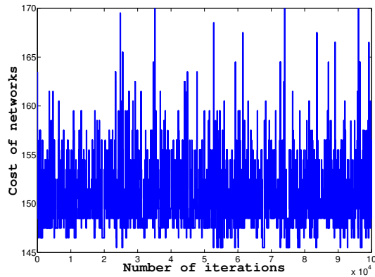
Figure 4: Sample path of network dynamics for \varepsilon = 0.01
