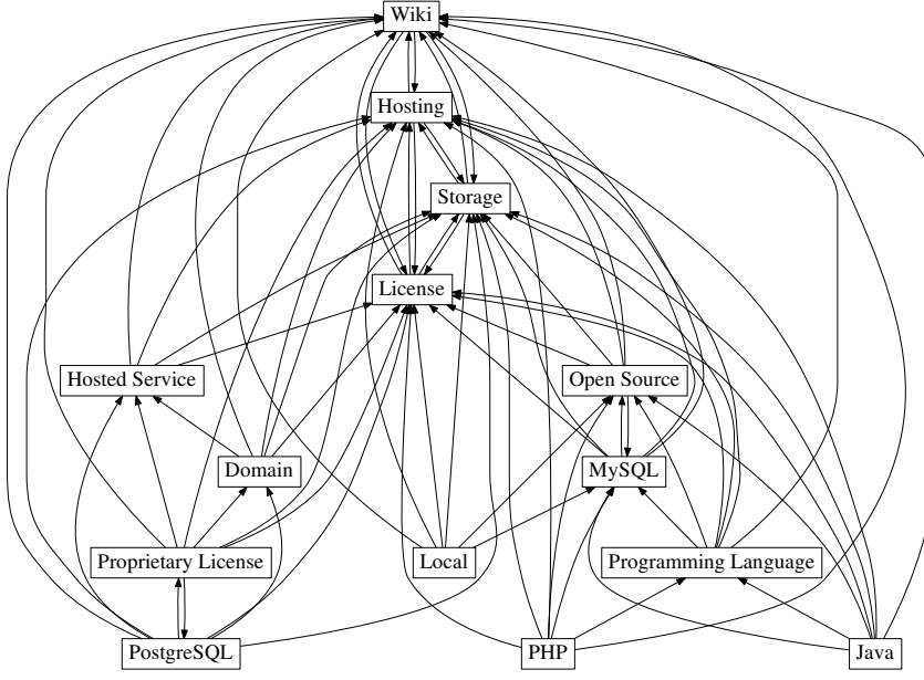
Fig. 4: Binary implication graph of the formula in Figure 3b
