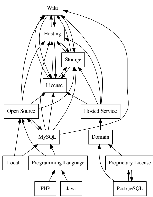
Fig. 5: Reduced binary implication graph of the graph in Figure 4
