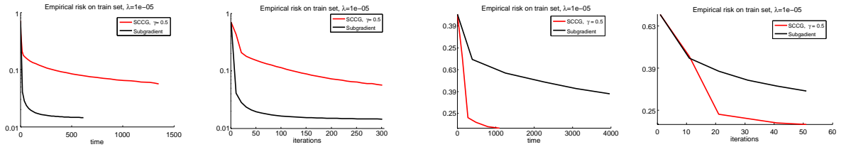
Figure 1: Comparison of empirical risk vs time (left of each box) and vs iterations number (right); \gamma = 0.5, \lambda = 10^{-5} , on MovieLens datasets: the small dataset for the two figures on the left-hand side, the medium dataset for the two on the right-hand side.
