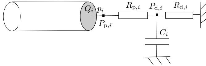
FIGURE 3. The RCR reduced model.
