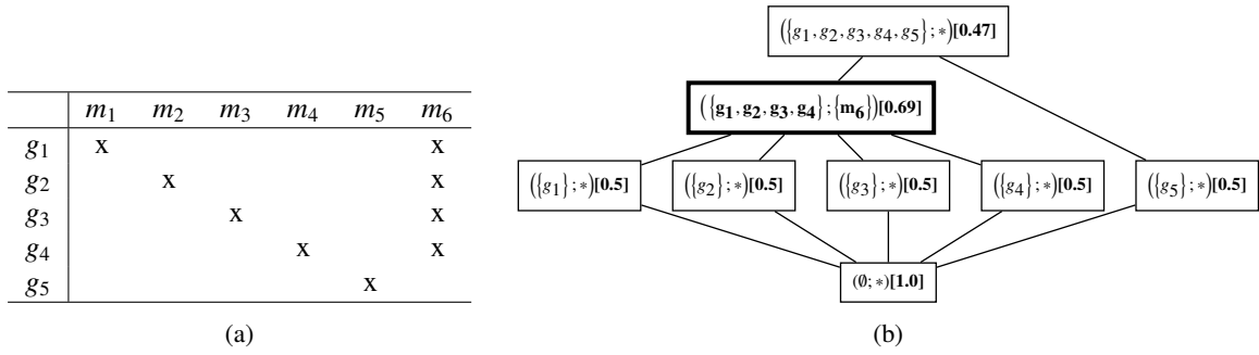
Fig. 1: (a) A toy formal context.
