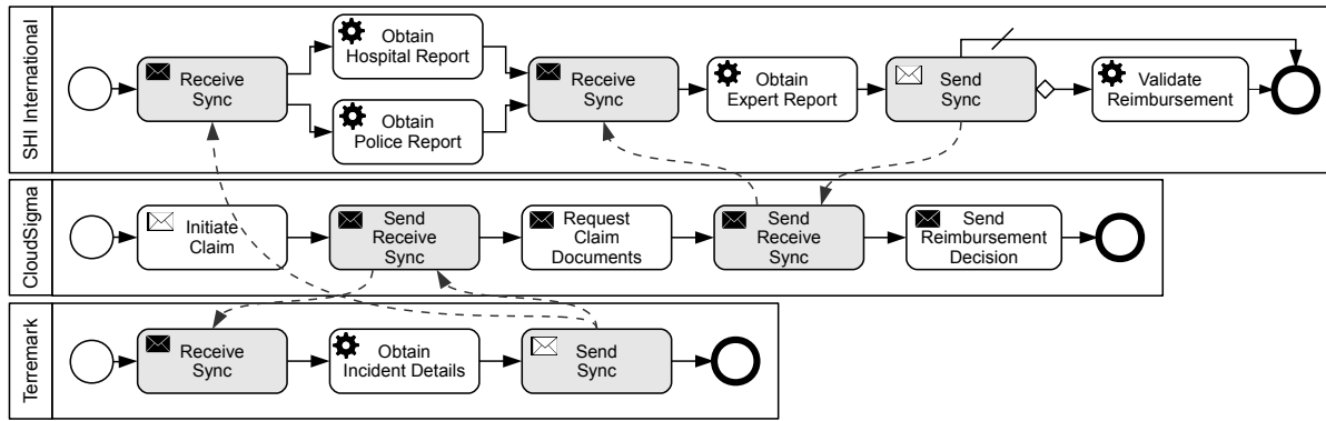
Fig. 4. A partitioned orchestration process.
