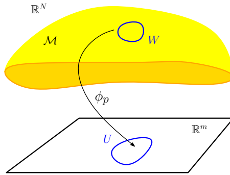
Figure 8.2: A local coordinate chart at a point p in \mathcal{M}
