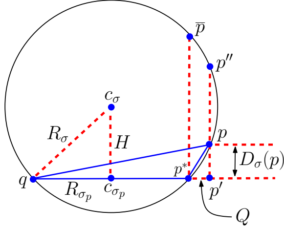
Figure 2.3: Refer to the proof of Lemma 2.3.1 (3), Case (c).
