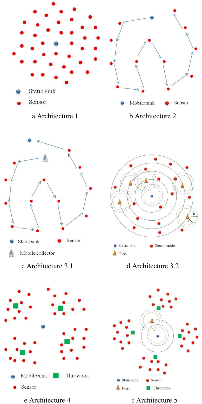
Figure 2: WSN Architectures.
