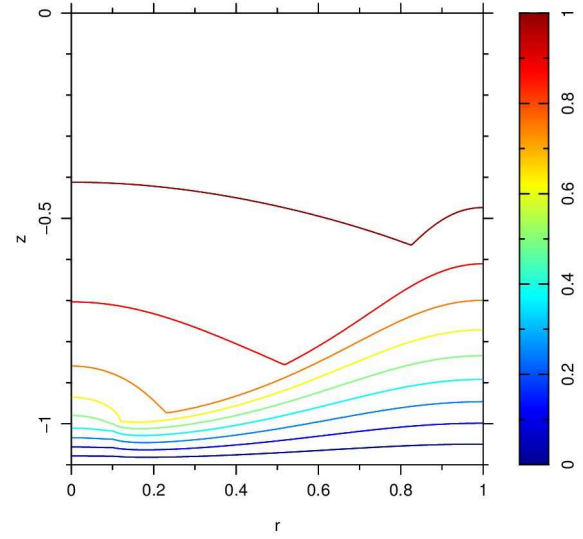
Fig. 5. The contour curves of the temperature obtained after a numerical computation on a 500x500 mesh.
