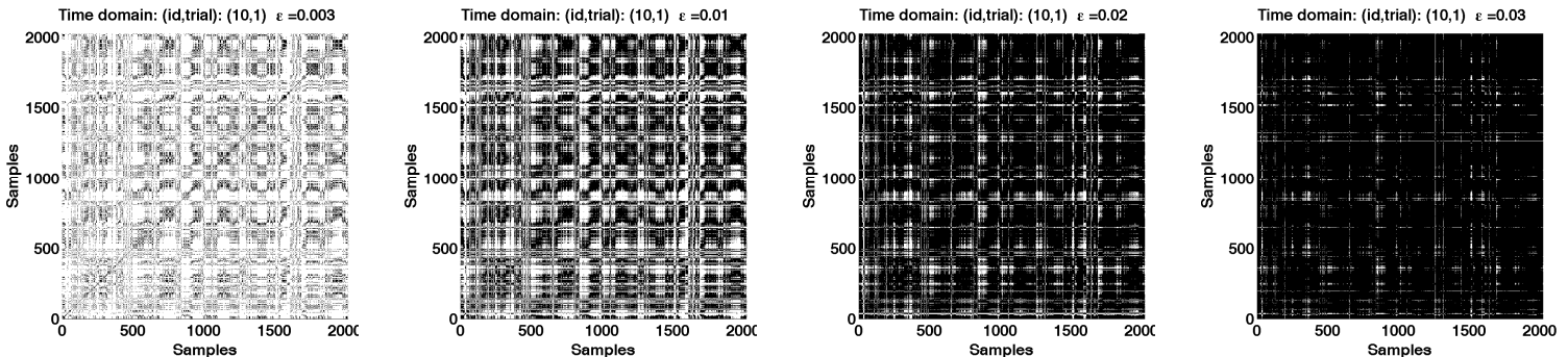
Fig. 1. Ferret measurements (time domain): recurrence plots obtained for the set of threshold values \epsilon \in \{0.003, 0.01, 0.02, 0.03\} .
