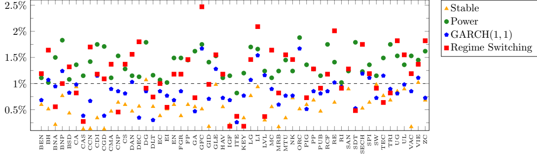
Figure 2: Violation ratios of 56 Euronext Paris stocks under the four estimation models.
