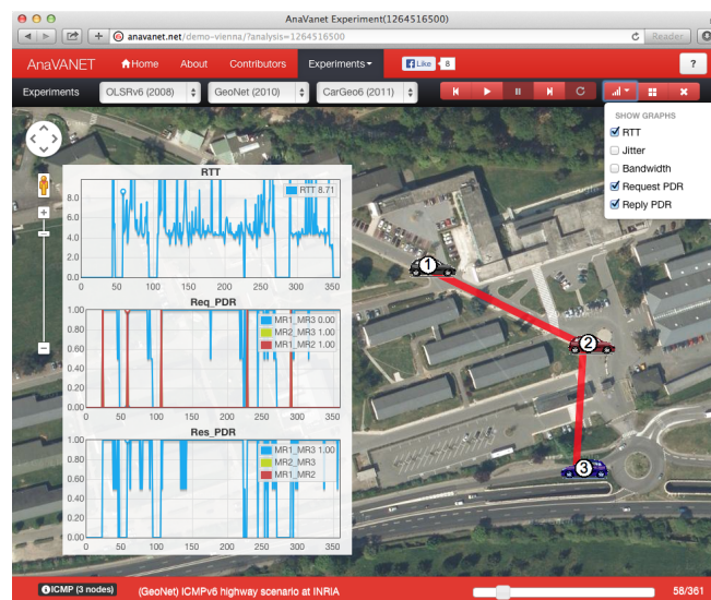
Figure 1. Screenshot of AnaVANET viewer
