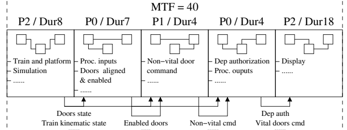
Figure 3. The partitional scheduling result of LOPHT.
