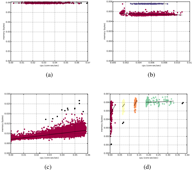
Fig. 3: Dependency of memory usage vs CPU consumption of four different jobs.
