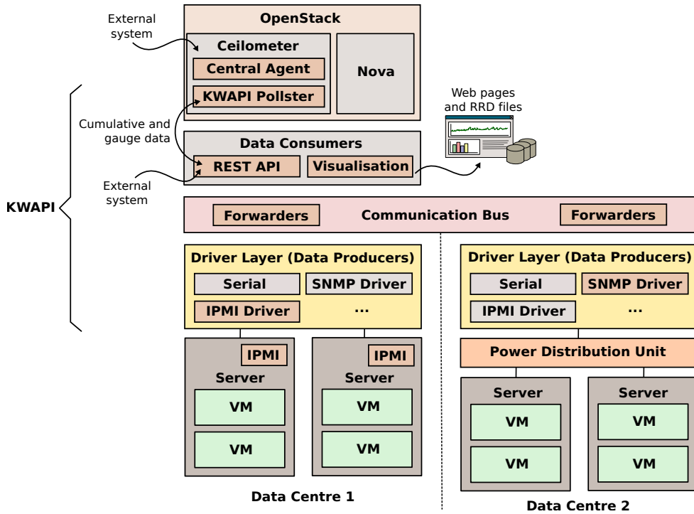
Fig. 2. Overview of KWAPI's architecture.
