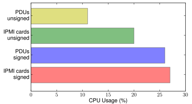
Fig. 5. Driver CPU usage under the evaluated scenarios.
