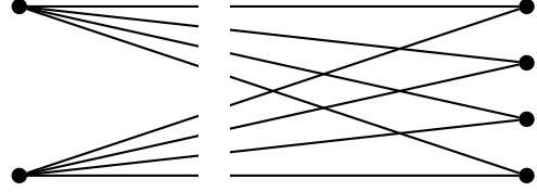
Figure 2: Complete bipartite graph K(2, 4) with weights p and q .
