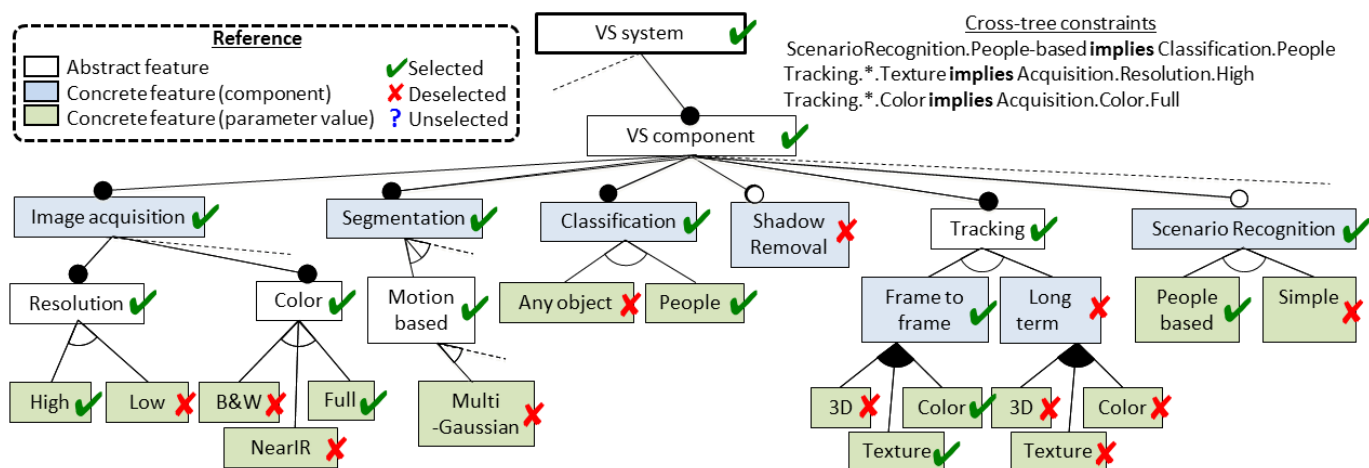
(b) Feature model full configuration of a video surveillance processing chain
