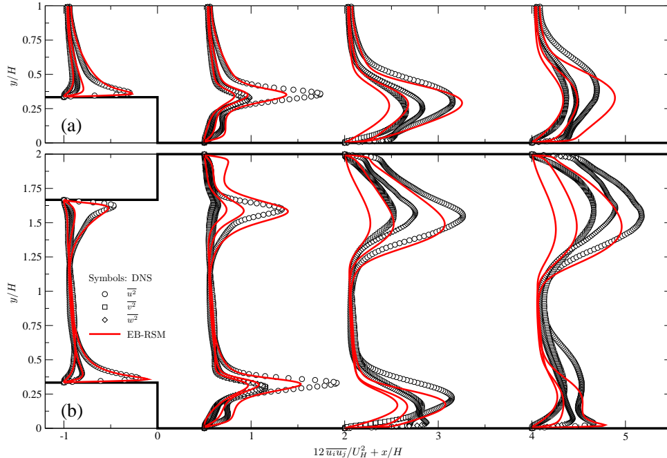
Figure 20: Channel with sudden expansion. Normal stress ( \overline{u^2} , \overline{v^2} , \overline{w^2} ) profiles. (a) Non-rotating case; (b) Rotating case.
