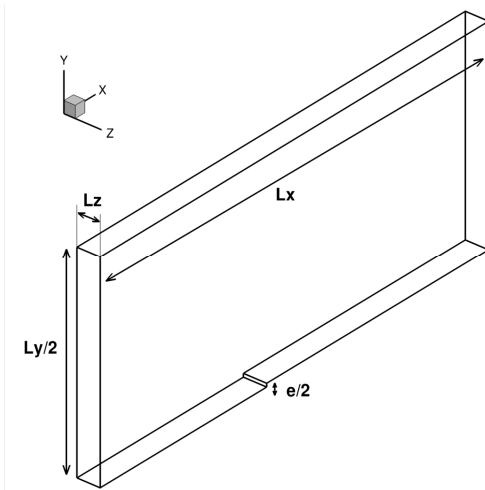
Figure 1 : Flow configuration
