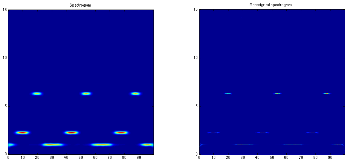
Figure 2.11: Spectrogram reassignment.
