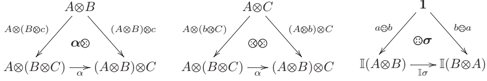
Fig. 8. Coherence diagrams for the virtual tensors
