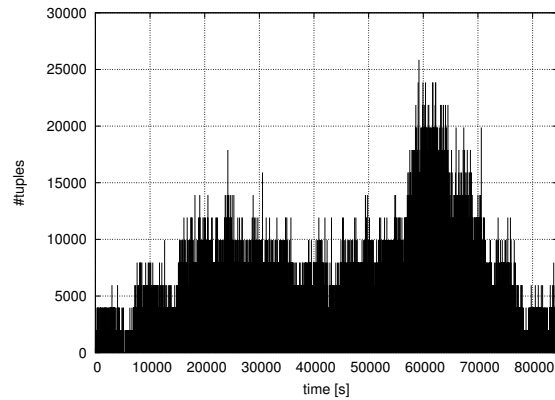
Figure 5: Maximum GPS data generation frequency registered in a single day by 30 million of users
