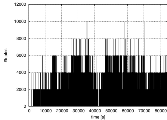
Figure 6: Minimum GPS data generation frequency registered in a single day by 30 million of users
