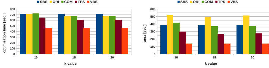
(a) otime results (in seconds).
