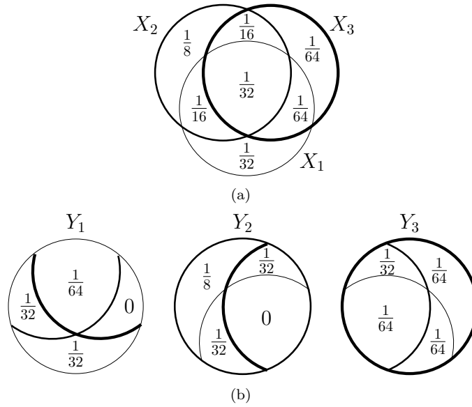
Figure 5: Disentangling Sets
