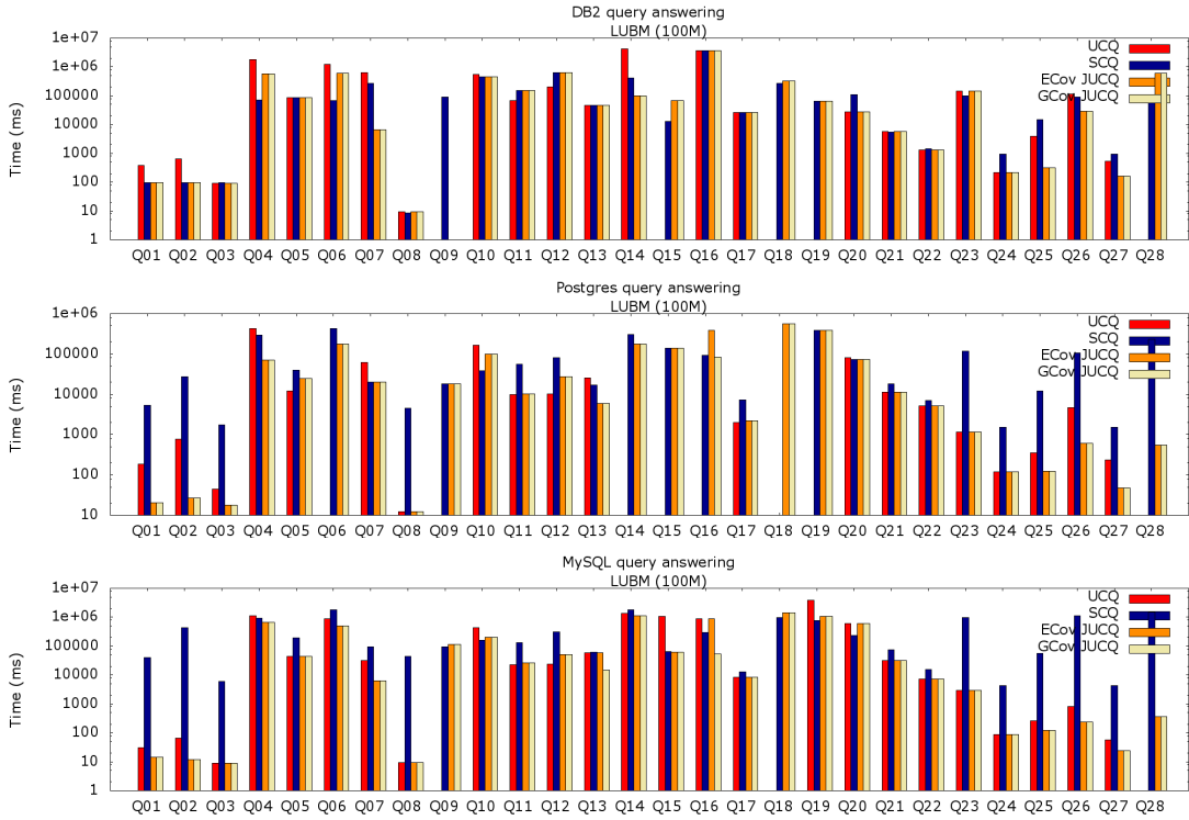
Figure 5: LUBM 100M query answering through UCQ, SCQ, ECov and GCov JUCQ reformulations, against DB2, Postgres and MySQL.
