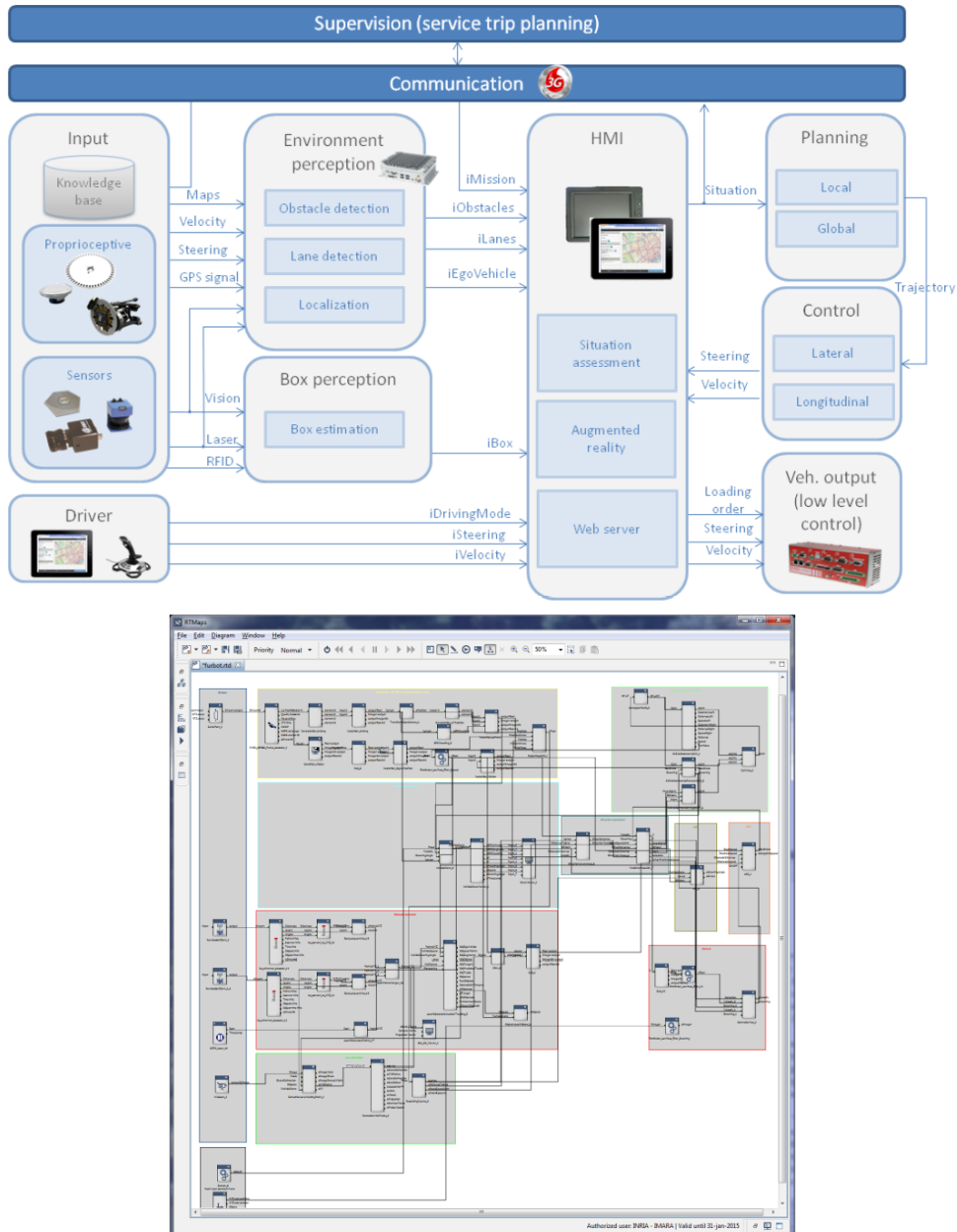
Figure 6 (a) General control architecture of the Furbot vehicle and (b) its implementation with the RTMaps software (see online version for colours)
