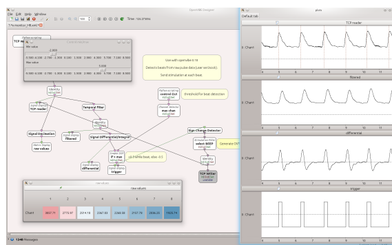
Figure 4: Signal processing of the BVP sensor with OpenViBE. A low-pass filtered and a first-derivative are used to detect heartbeats.
