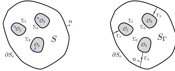
FIGURE 1. The geometry of the domain S .
