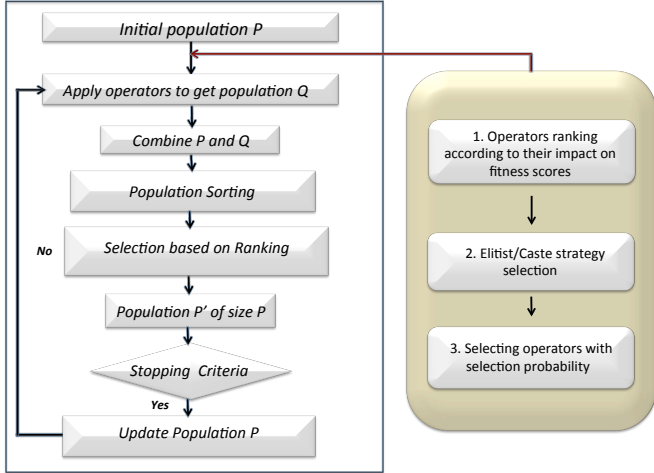
Fig. 1: Sputnik Workflow
