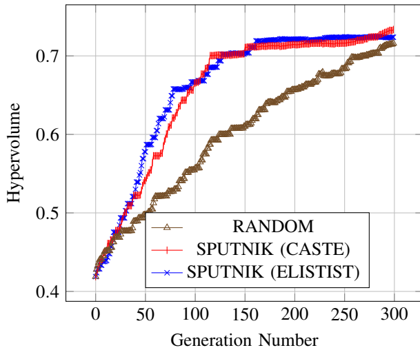
Fig. 2: Hypervolume: Sputnik (Elitist & Caste) versus Random Selection
