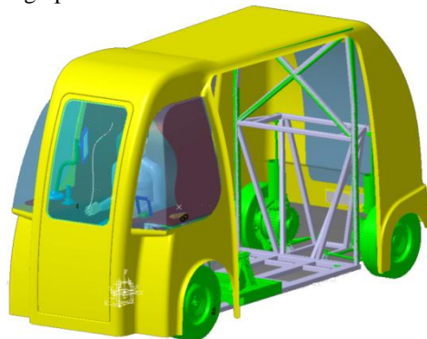
Figure 1: the Furobot prototype
