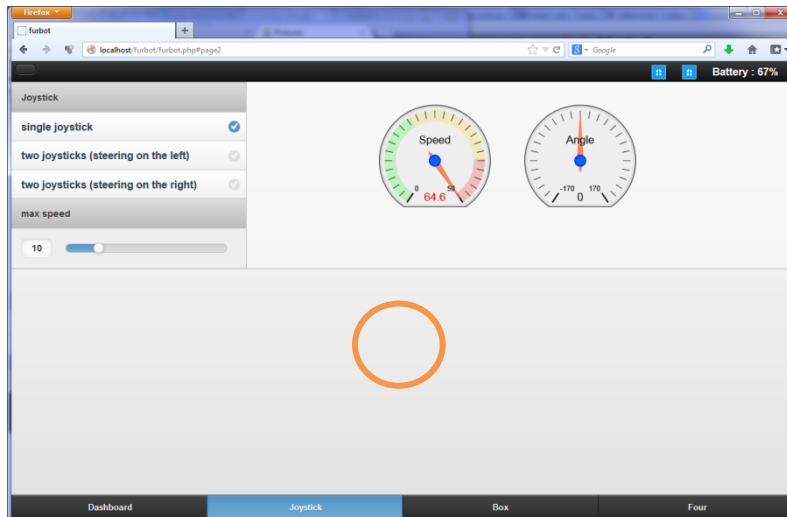
Figure 14: Virtual joystick
