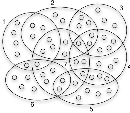
Figure 8: Hypergraph \mathcal{H} = (\mathcal{V}, \mathcal{E}) with \mathcal{E} = \{e_1, e_2, e_3, e_4, e_5, e_6, e_7\} . A hyperedge with i \in \llbracket 1, 7 \rrbracket represents e_i \in \mathcal{E} . The auxiliary instance (U, S) of the weighted set packing problem from \mathcal{H} is such that U = \{e_1, e_2, e_3, e_4, e_5, e_6, e_7\} and S = \{\{e_1, e_2\}, \{e_1, e_6\}, \{e_1, e_7\}, \{e_2, e_3\}, \{e_2, e_4\}, \{e_2, e_7\}, \{e_3, e_4\}, \{e_3, e_7\}, \{e_4, e_5\}, \{e_4, e_7\}, \{e_5, e_6\}, \{e_5, e_7\}, \{e_6, e_7\}, \{e_1, e_2, e_7\}, \{e_1, e_6, e_7\}, \{e_2, e_3, e_7\}, \{e_2, e_3, e_4\}, \{e_3, e_4, e_7\}, \{e_2, e_4, e_7\}, \{e_4, e_5, e_7\}, \{e_5, e_6, e_7\}, \{e_2, e_3, e_4, e_7\}\} . Furthermore, w_{\{e_1, e_2\}} = 6 , w_{\{e_1, e_6\}} = 2 , w_{\{e_1, e_7\}} = 4 , w_{\{e_2, e_3\}} = 6 , w_{\{e_2, e_4\}} = 3 , w_{\{e_2, e_7\}} = 6 , w_{\{e_3, e_4\}} = 7 , w_{\{e_3, e_7\}} = 1 , w_{\{e_4, e_5\}} = 4 , w_{\{e_4, e_7\}} = 4 , w_{\{e_5, e_6\}} = 2 , w_{\{e_5, e_7\}} = 4 , w_{\{e_6, e_7\}} = 6 , w_{\{e_1, e_2, e_7\}} = 9 , w_{\{e_1, e_6, e_7\}} = 7 , w_{\{e_2, e_3, e_7\}} = 7 , w_{\{e_2, e_3, e_4\}} = 10 , w_{\{e_3, e_4, e_7\}} = 8 , w_{\{e_2, e_4, e_7\}} = 7 , w_{\{e_2, e_3, e_4\}} = 5 , w_{\{e_5, e_6, e_7\}} = 8 , and w_{\{e_2, e_3, e_4, e_7\}} = 11 . For instance, \{e_2, e_3, e_4\} \in S and w_{\{e_2, e_3, e_4\}} = 10 because |e_2 \cap e_3 \cap e_4| = 3 and \max(w_{\{e_2, e_3\}}, w_{\{e_2, e_4\}}, w_{\{e_3, e_4\}}) - 3 = 4 . The packing C^* = \{\{e_1, e_2\}, \{e_3, e_4\}, \{e_5, e_6, e_7\}\} is such that \sum_{c \in C^*} w_c = 21 and is optimal for the weighted set packing problem for (U, S) . From Theorem 21, we get that \max_{local}^* = \max_{global}^* = 21 .
