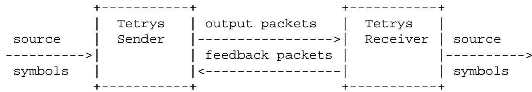
Figure 1: Tetrys Architecture.
