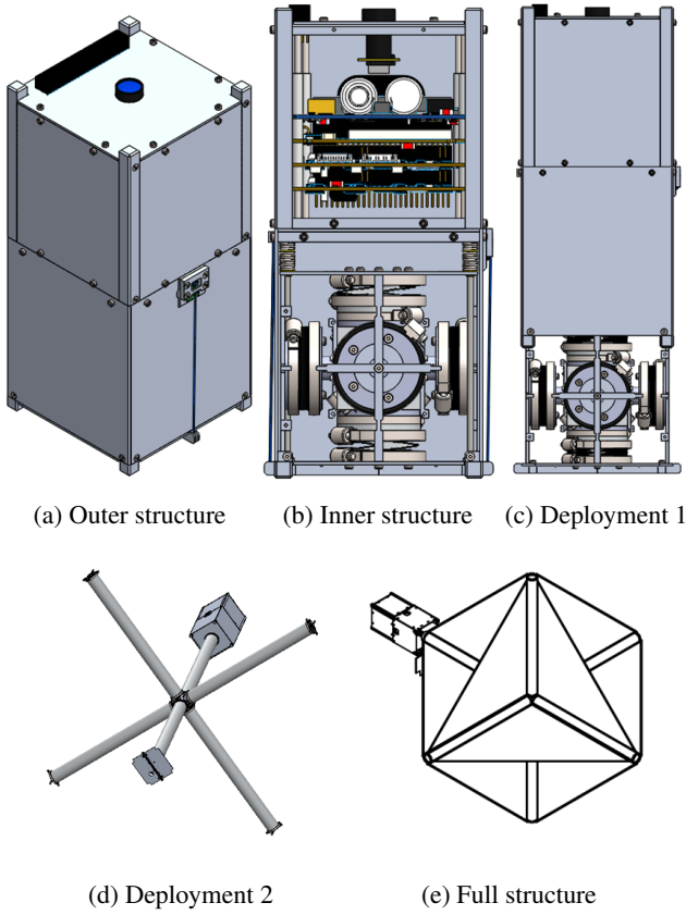
Fig. 7: Net Cubesat (DS-1): Structure
