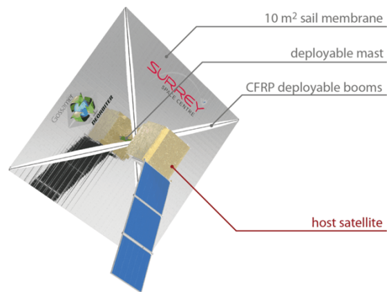
Fig. 23: Dragsail Concept.
