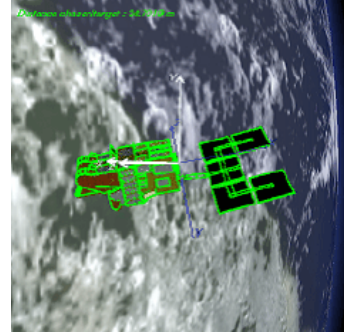
Fig. 18: 2D / 3D Matching.
