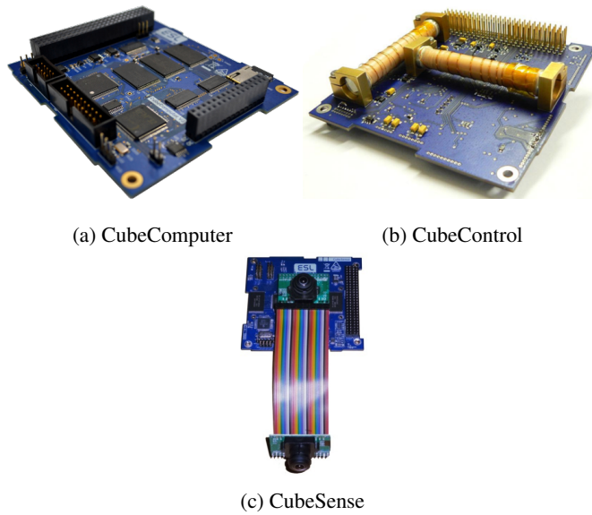
Fig. 10: Avionics: Individual Boards
