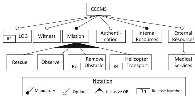
Fig. 1 Partial feature model for the CCCMS SPL
