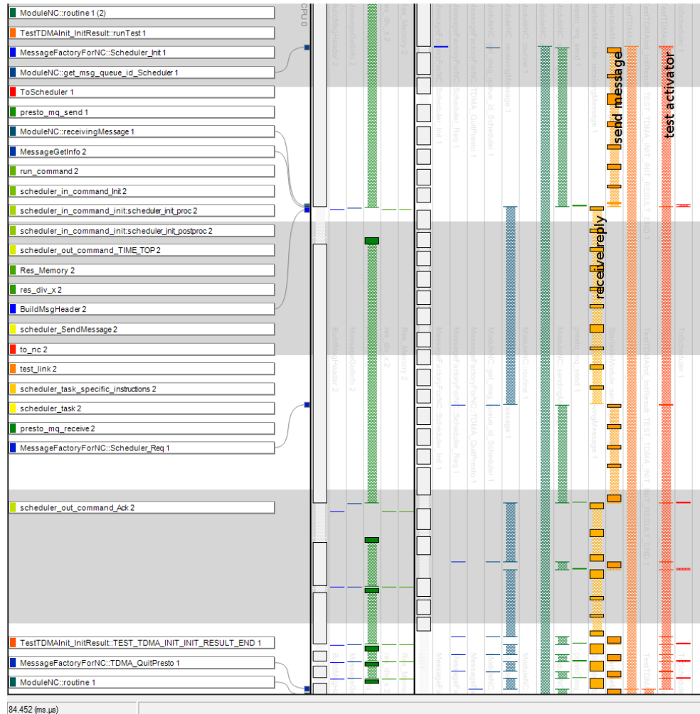
Figure 7 RapiTrace Viewer showing ‘function view’ in the TDMA radio case study.
