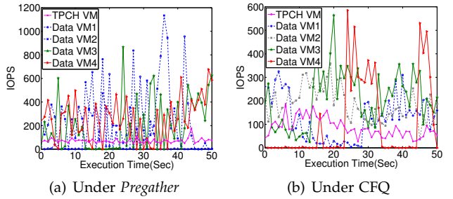
Fig. 11: The changes of throughput of Data VMs and TPC-H VM
