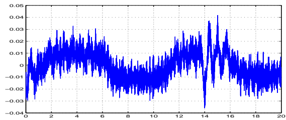
(h) Implicit. sign(\sigma_{k+1}) . G = 10^5 , h = 5\text{ms} .
