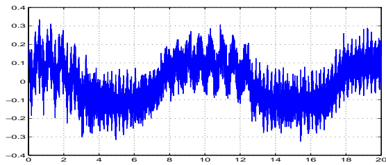
(g) Implicit. sign(\sigma_{k+1}) . G = 10^4 , h = 5\text{ms} .
