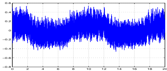
(e) Implicit. sign(\sigma_{k+1}) . G = 10^4 , h = 2\text{ms} .
