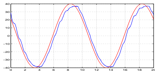
(f) h = 15\text{ms} . Implicit method.
