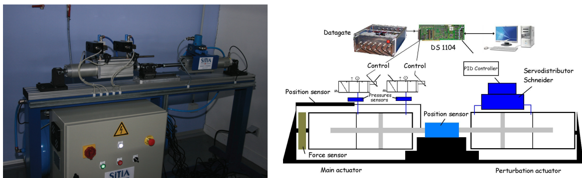
Figure 1: [18] Photography and scheme of the electropneumatic system.
