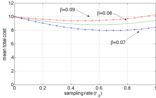
Figure 5. Varying the infection rate per contact, \beta .
