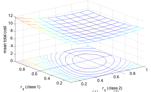
Figure 7. Asymmetric setup with c_v^{(1)} = 7, c_v^{(2)} = 14 .
